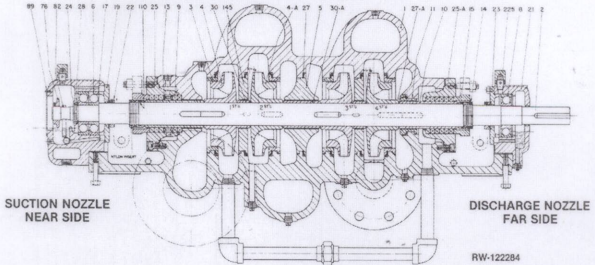
CLOCKWISE ROTATION VIEWED FROM OUTBOARD END OF PUMP
