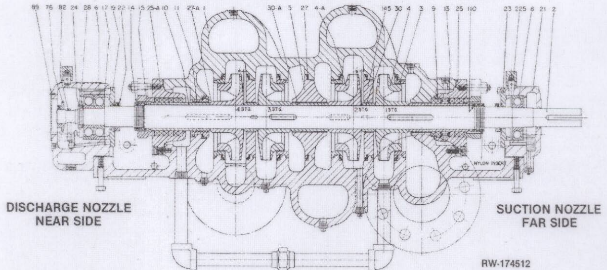
COUNTER CLOCKWISE VIEWED FROM OUTBOARD END OF PUMP
